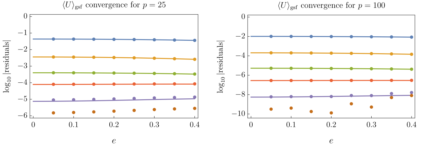
FIG. 2. Comparison of our PN expressions with numerical data from Table II of Akcay et al. [18]. Dots are numerical values and lines are our analytic calculations. The top row is \log_{10} of the absolute value of the full \langle U \rangle_{\text{gsf}} . Successive rows show residuals after subtracting each term in the PN series. The consistency of our agreement out to e = 0.4 is only possible because of our re-summation of the small- e expansion. Unevenness of the final residuals for p = 100 is likely a numerical artifact.
