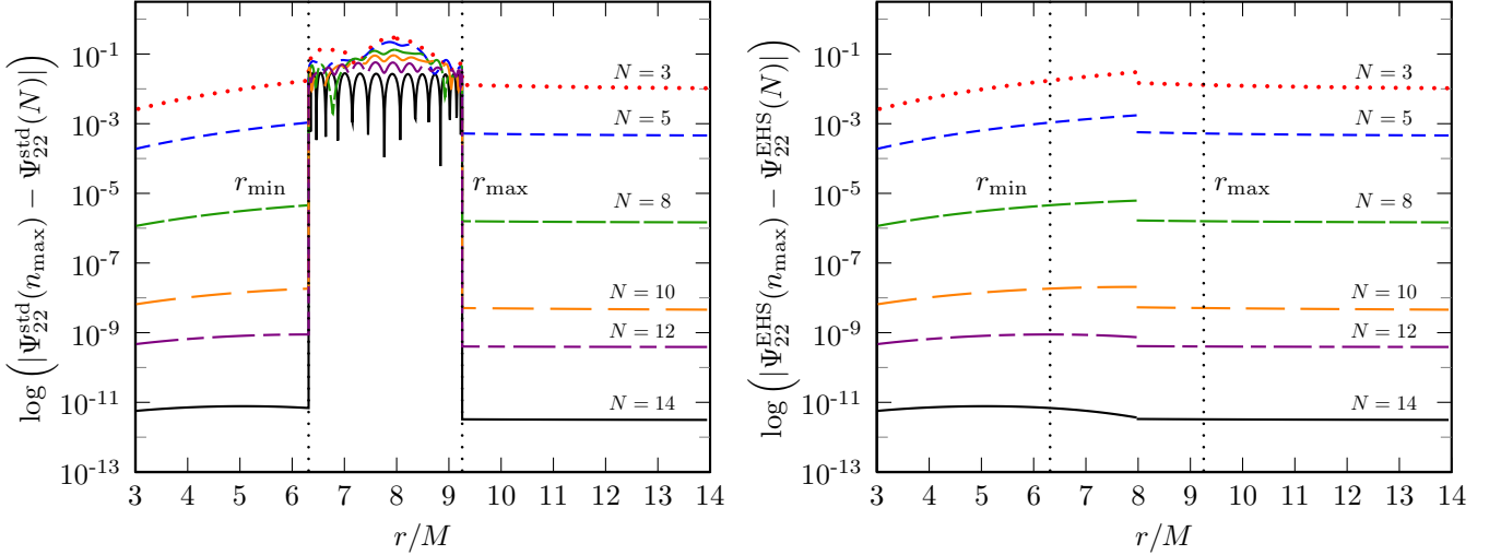
FIG. 4: A plot of the convergence of the master function using the two methods. For a particle orbiting with p = 7.50478 and e = 0.188917 at t = 51.78M we compute the master function \Psi_{22}(n_{\text{max}}) by summing over modes ranging from -n_{\text{max}} \leq n \leq n_{\text{max}} for n_{\text{max}} = 15 . We plot the log of the difference between \Psi_{22}(n_{\text{max}}) and the partial sum \Psi_{22}(N) , for different N < n_{\text{max}} . For the standard approach (left), we see exponential convergence in the homogeneous region, but only algebraic convergence in the region of the source. The method of extended homogeneous solutions (right) yields exponentially converging results at all points outside and inside the region of the source. The method of extended homogeneous solutions gives exponential convergence for \partial_r \Psi_{\ell m}^{\text{EHS}} as well.
